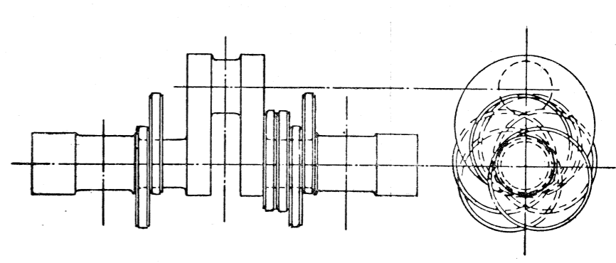
Fig. 8 Crank Axle and Eccentric Sheaves, N.E.R.
