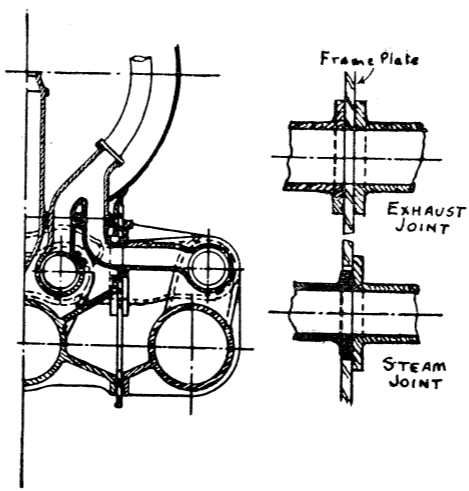
Fig. 6 - Cross Section of Cylinders, Cal. Rly. and Details of Joints.
